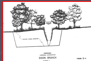
Alternate 4 Channel Cross Section
